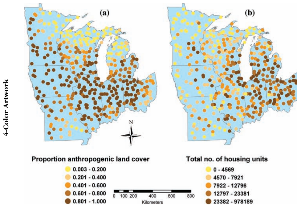
Figure 2. The (a) proportion of anthropogenic land cover and (b) total number of housing units present in each survey landscape in the midwestern United States.
