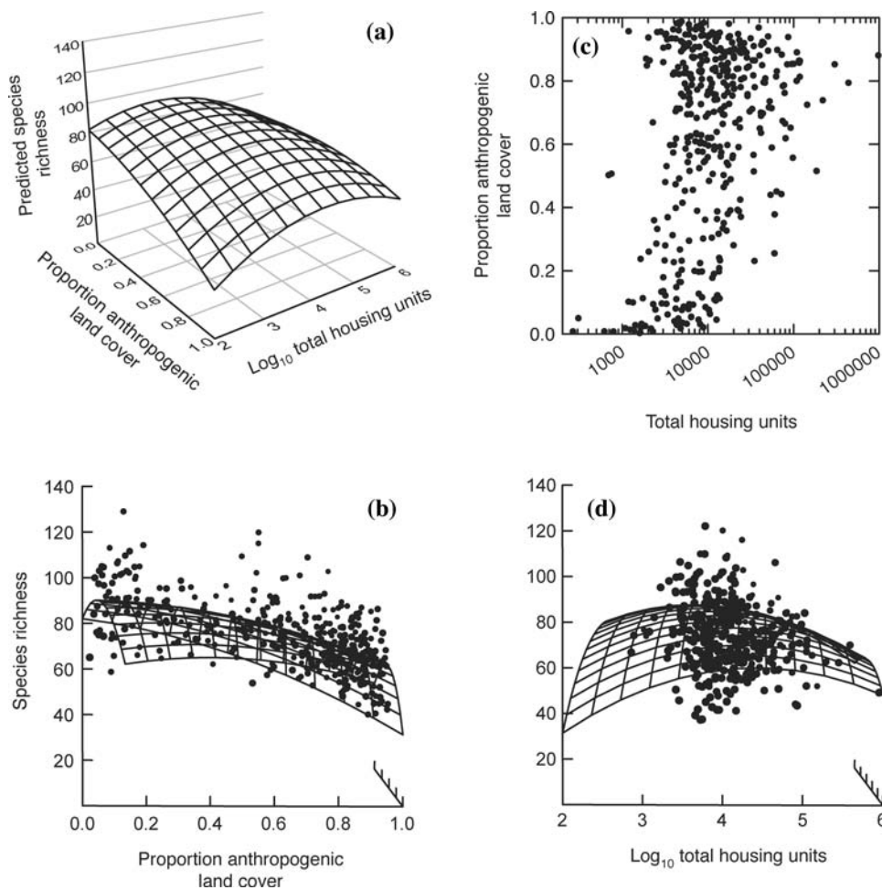
Figure 4. (a) Predicted native species richness in relation to the proportion of anthropogenic land cover and the log 10 total number of housing units on the landscape. (b) Predicted (surface) and observed (●; i.e., Comdyn estimates) species richness in relation to anthropogenic land cover. (c) Location of landscapes on the anthropogenic land-cover and housing-unit gradient (log scale). (d) Predicted (surface) and observed (●; i.e., Comdyn estimates) species richness in relation to log 10 total housing units.
