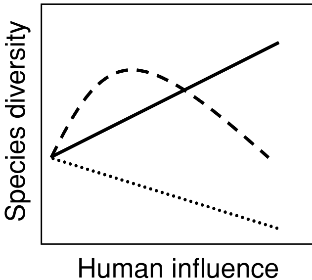
Figure 1. Competing hypotheses that explain the relationships between species diversity and human influence (i.e., population, houses): productivity (solid line), intermediate disturbance (dashed line), and ecosystem stress (dotted line).
