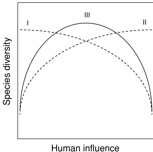
Figure 3. Illustration of how quadratic models relate to the productivity, intermediate-disturbance, and ecosystem-stress hypotheses. If the parabola's apex occurs at the x-axis (I), where human influence is the lowest, the relationship is an ecosystem-stress relationship. If the parabola's apex occurs at or near the greatest level of human influence (II), the relationship is a productivity relationship. If the parabola's apex occurs in the mid ranges of human influence (III), the relationship is an intermediate-disturbance relationship.
