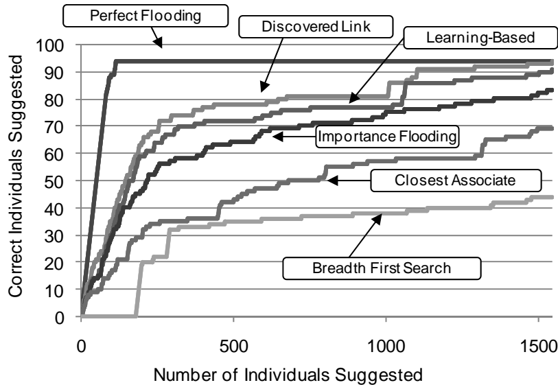
Figure 5. Fraud/Meth Results – Importance flooding (Discovered Link, Learning-Based, and Importance Flooding) outperformed the other approaches. Discovered links and user feedback improved the results.
