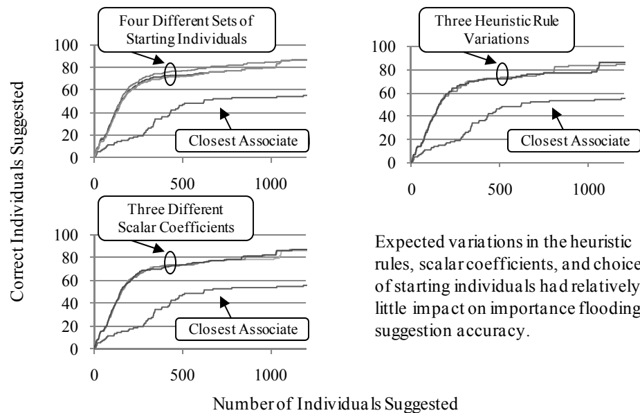
Figure 7. Fraud/Meth Results Given Parameter Variations
