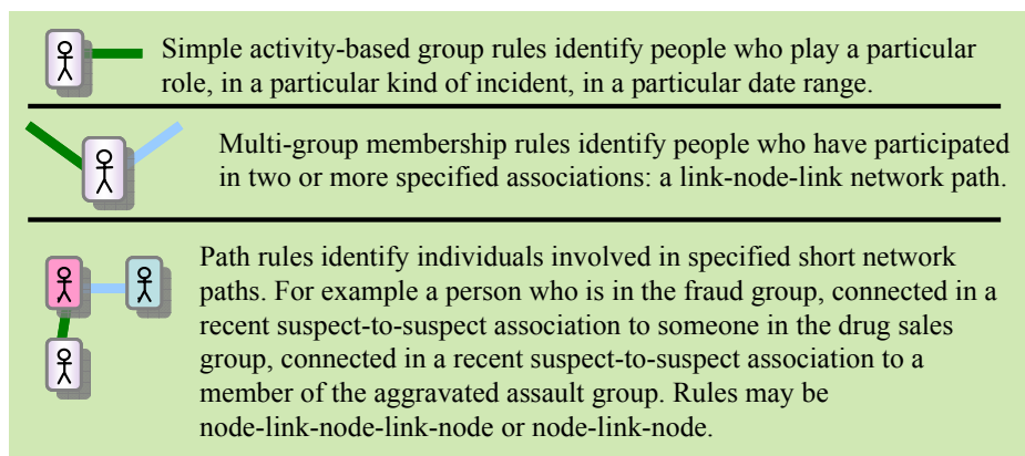
Figure 3. Three Types of Initial Importance Rules
