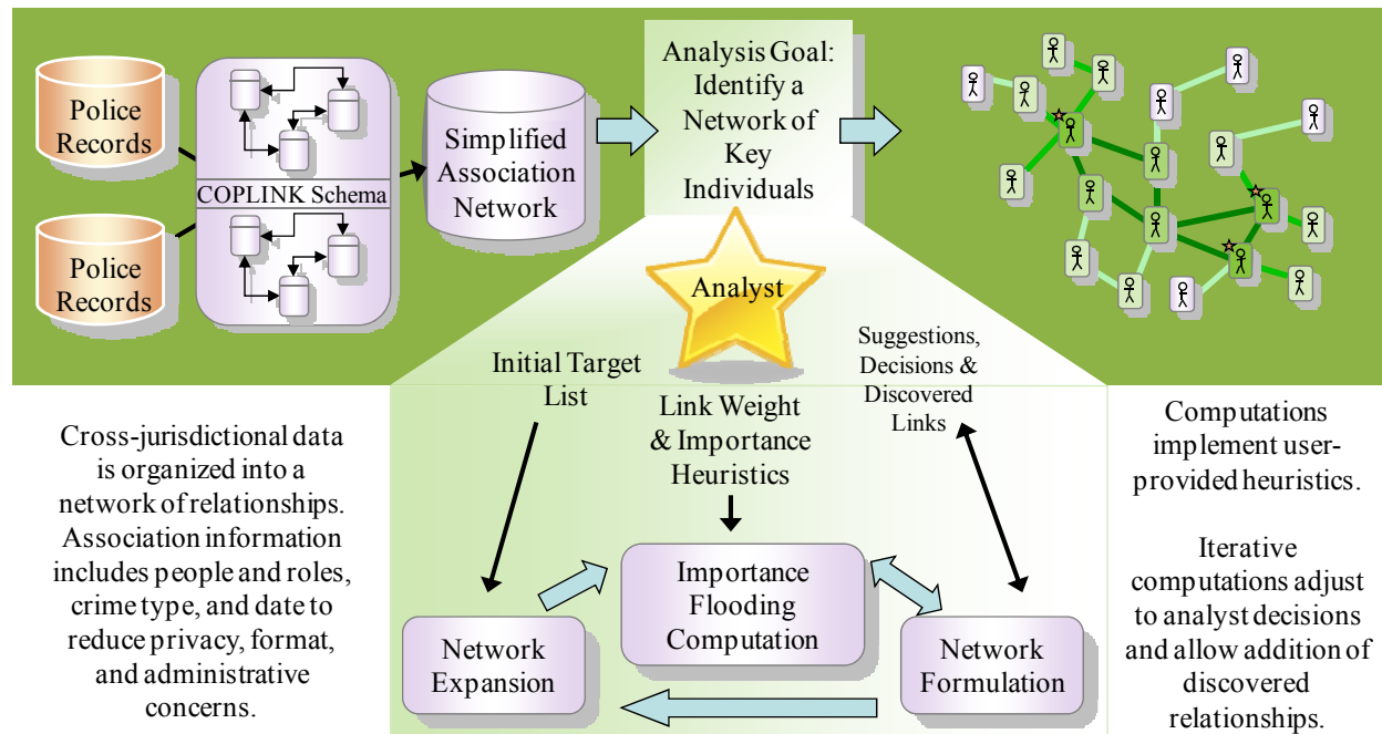
Figure 2. Relations are extracted and formatted to form a large criminal activity network, the importance flooding algorithm iteratively suggests potentially interesting individuals as leads, and the analyst constructs a link chart. In our experiments, data was extracted from the COPLINK systems of two police agencies.
