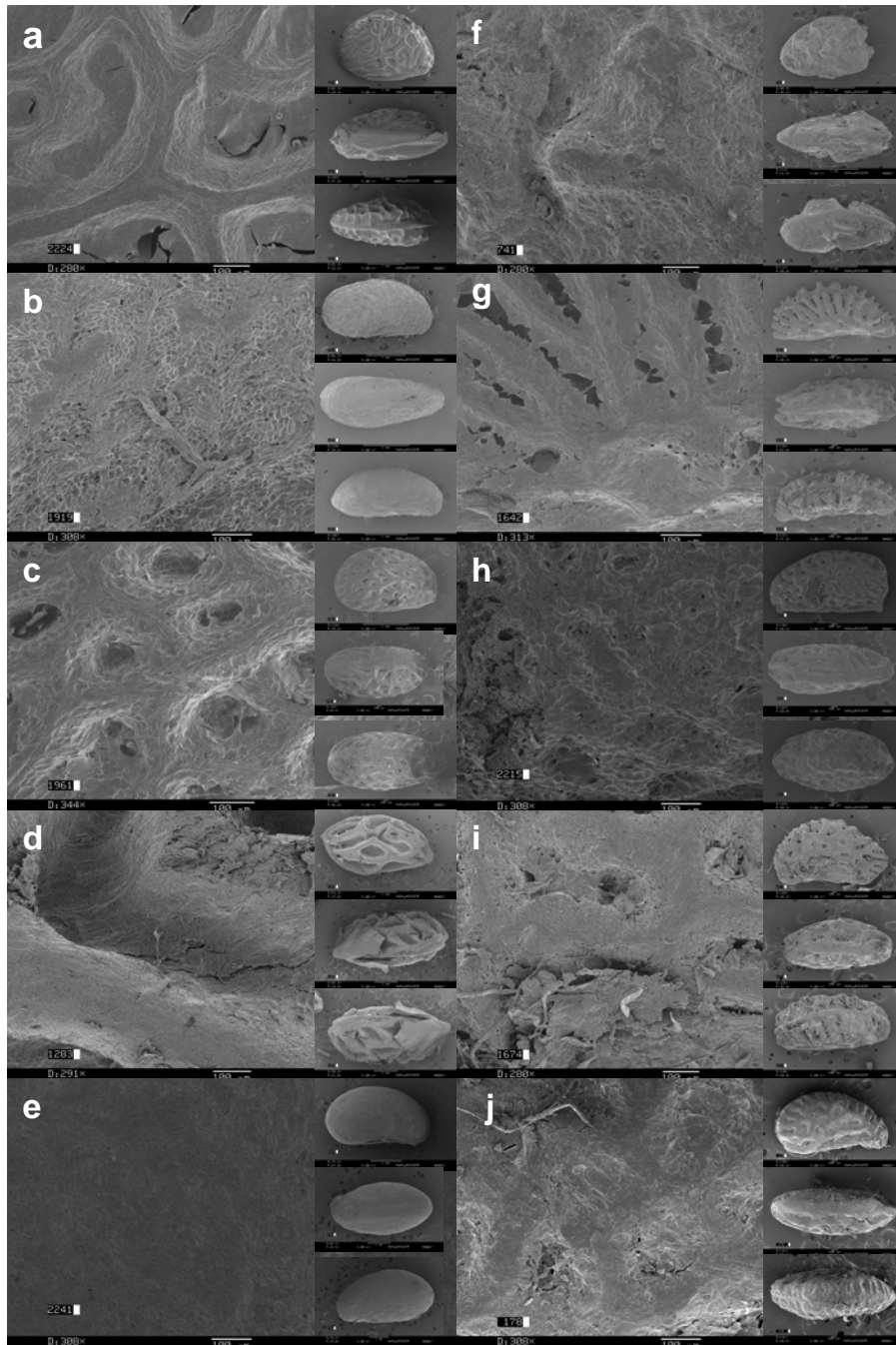
Fig. 1. SEM images: For each letter (a-j) there is a surface view in higher magnification (the scales are shown below each) with smaller images of (upper) seed overview, (middle) view of a micropylar on the raphal region and (lower) view of a seed edge (back side of raphal region). a. Subg. Rubus ( R. lacinatus ), b. Subg. Cyclactis ( R. arcticus ), c. Subg. Idaeobatus ( R. aurantiacus ), d. Subg. Lampobatus ( R. bogotensis ) e. Subg. Chamaebatus ( R. chamaemorus ), f. Subg. Michranthobatus ( R. schimiloides ), g. Subg. Malachobatus ( R. multibracteatus ), h. Subg. Michranthobatus ( R. odoratus ), i. Subg. Dalibardastrum ( R. tsangorum ), j. Subg. Chamaebatus ( R. hayata-koizumii ).
